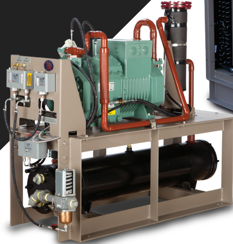
Typical Severe Duty Water Cooled Condenser
